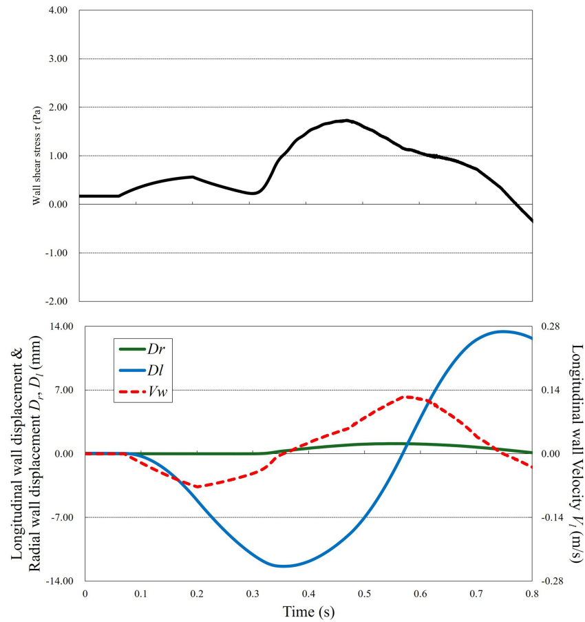
Fig. (9). WSS distribution and wave propagation are shown in the arterial model. The WSS T , radial wall displacement D_r , longitudinal wall displacement D_l , and longitudinal wall velocity V_t observed at z = 1,550 mm. (a) \lambda = 12.5 mm; (b) \lambda = 250 ms; and (c) \lambda = 500 ms.
