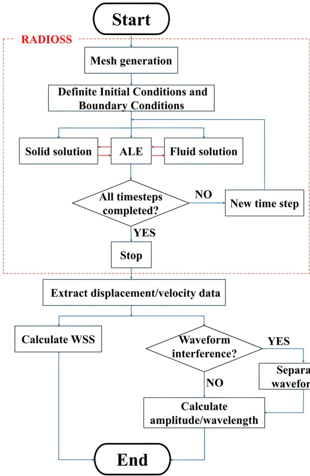
Fig. (4). Flowchart showing pre-processing to post-processing of simulations.
