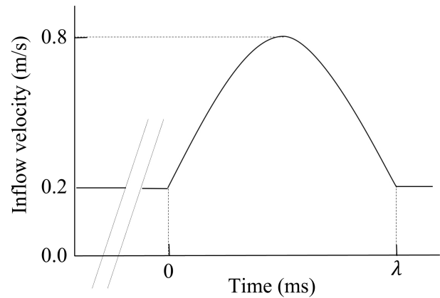
Fig. (3). Inlet boundary conditions.
