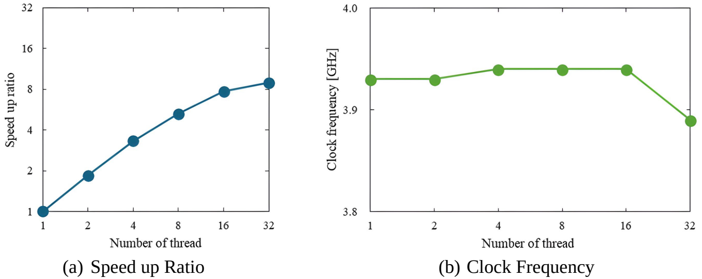
Fig. (2). (a) Speed up ratio with increasing number of threads. (b) Clock frequency at each number of threads.
