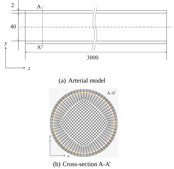
Fig. (1). (a) Arterial model used for the simulations. (b) Cross-section of the arterial model.
