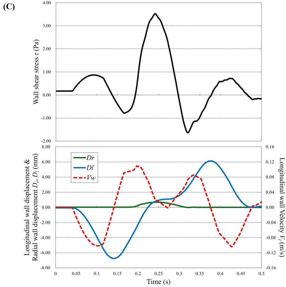
Fig. (6). WSS distribution and wave propagation are shown in the arterial model. The WSS \tau , radial wall displacement D_r , longitudinal wall displacement D_l , and longitudinal wall velocity V_l observed at z = 1550 mm. (a) E = 0.5 MPa; (b) E = 1.0 MPa; and (c) E = 1.5 MPa.
